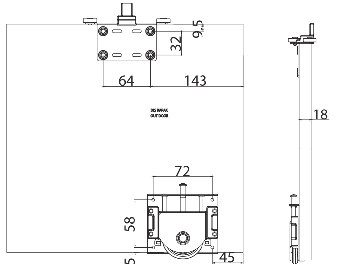
ALT RAY
