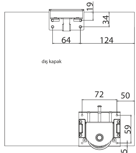
ALT RAY
